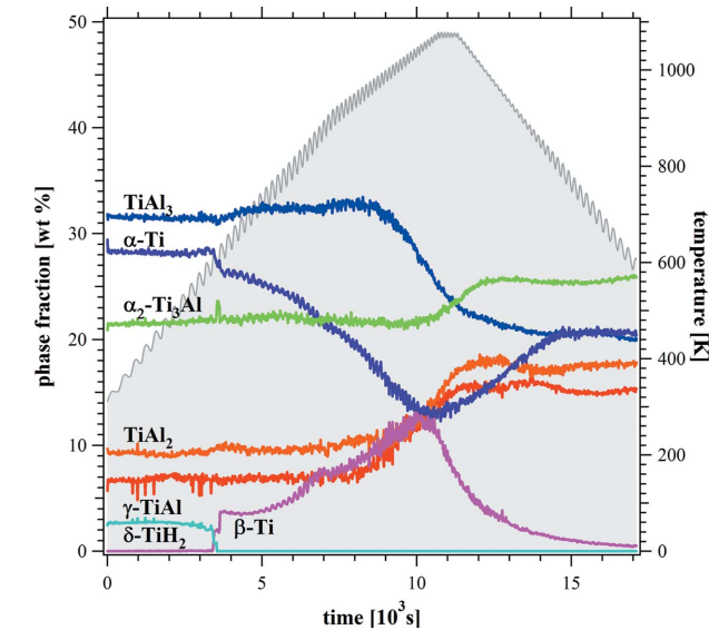
Figure 4 Weight fractions of the detected phases as a function of time (temperature) during the in situ scan as obtained by Rietveld refinement analysis in the ball-milled sample.
