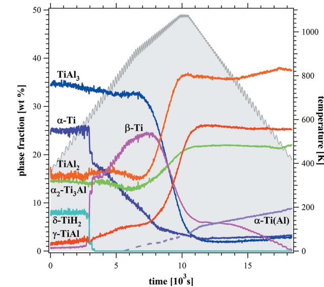
Figure 5 Weight fractions of the detected phases as a function of time (temperature) during the in situ scan as obtained by Rietveld refinement analysis in the raw sample.
